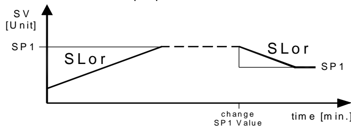
Example with start from values lower than SP1 and with decreasing of SP1.
