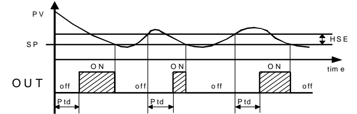
Example "Ptd" with "Fun" = Cool
