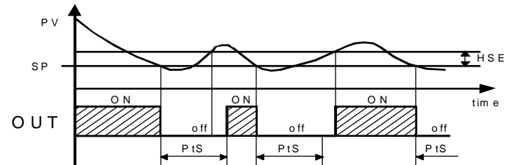
Example "PtS" with "Fun" = Cool
